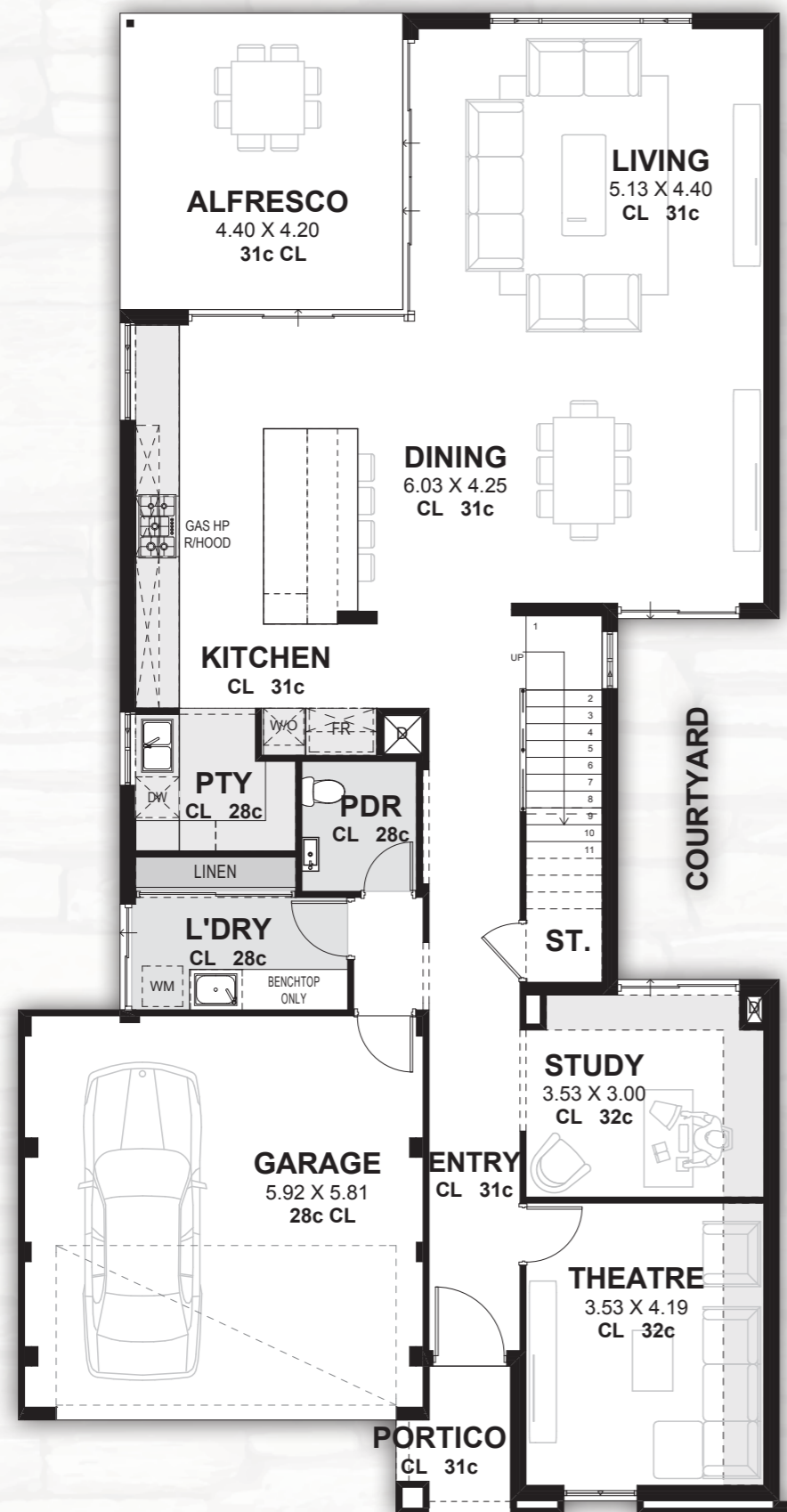
GROUND FLOOR
