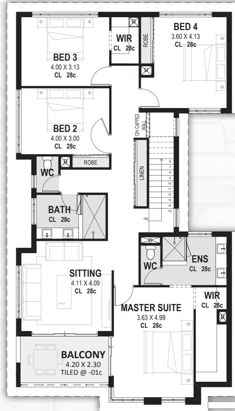
UPPER FLOOR
