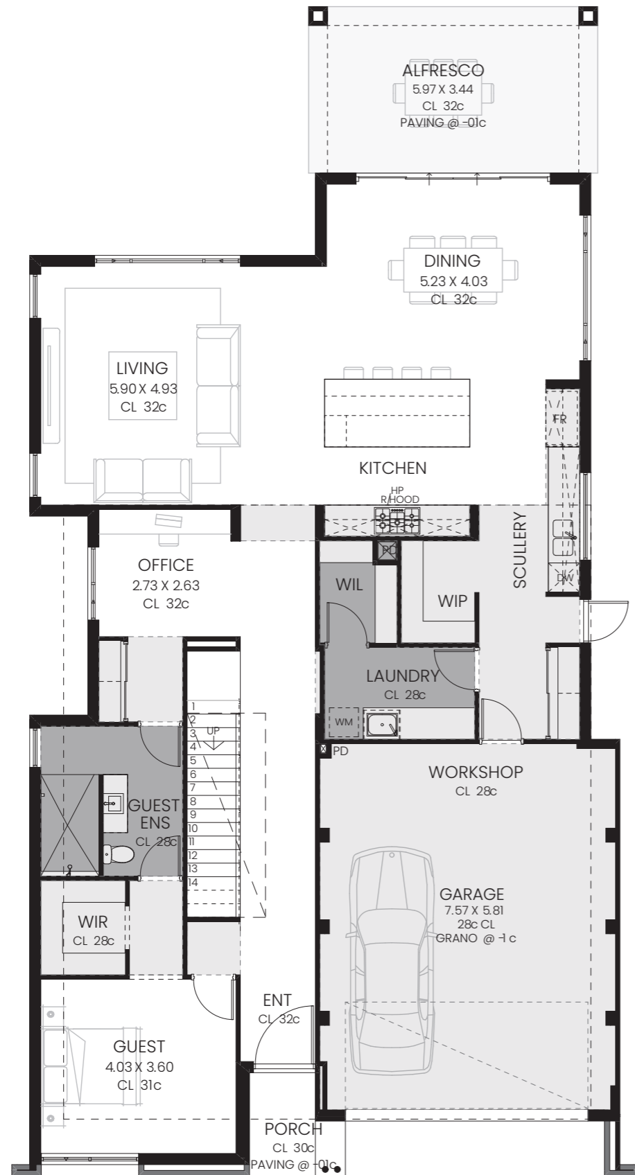
GROUND FLOOR
