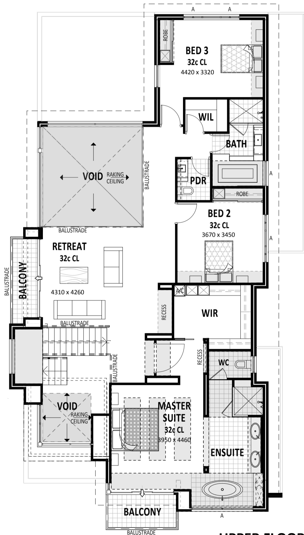
UPPER FLOOR
